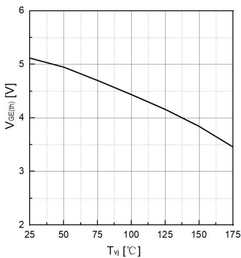
Fig 5. Typical V_{GE(th)} as a function of T_{vj}
